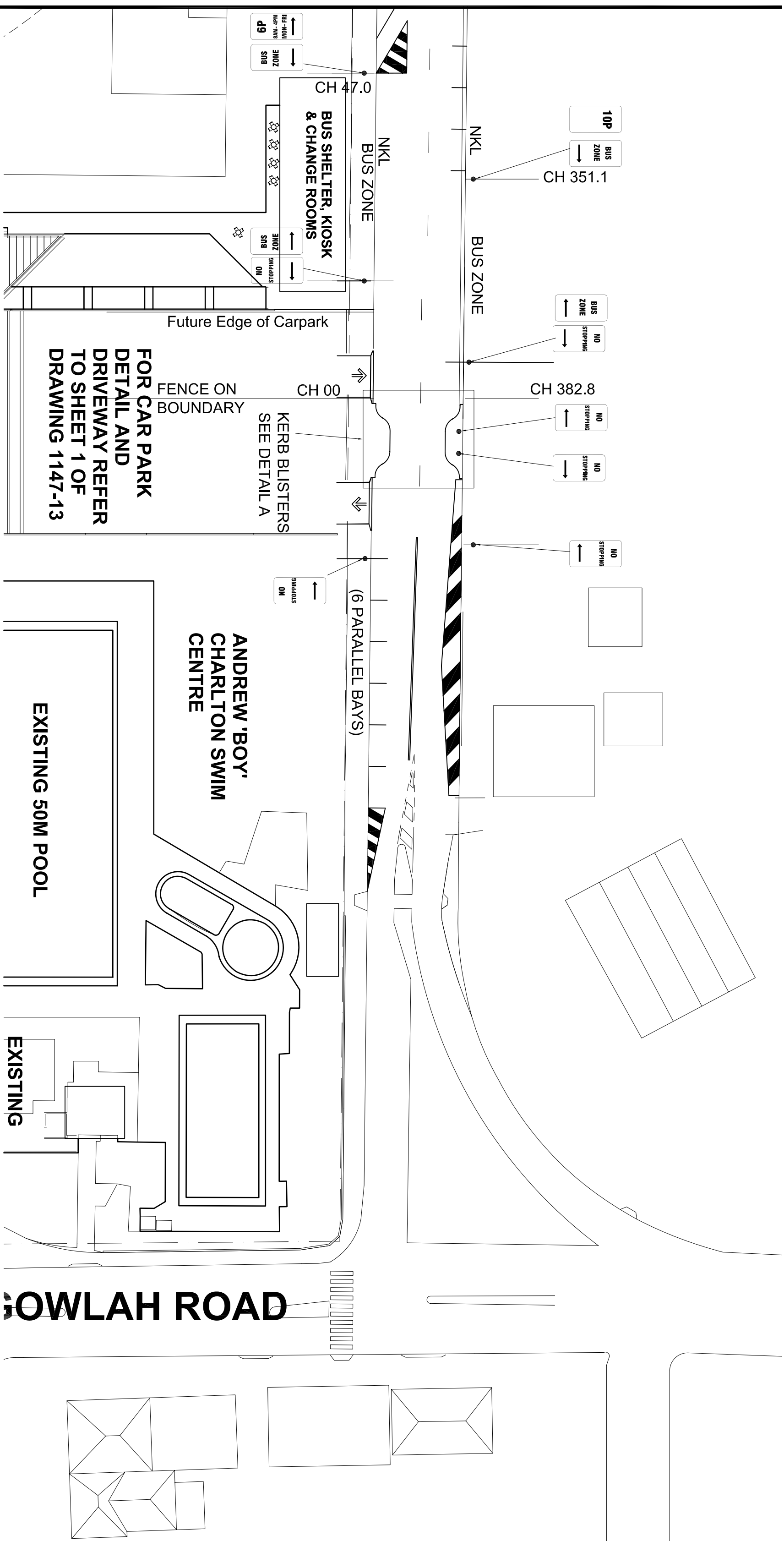
PLAN KERB BLISTERS DETAIL A SCALE 1:200
